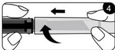
Screw the barrel back on
